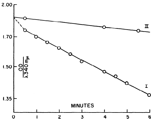
FIG. 5. Oxidation of DPNH by homogenates of bovine thrombocytes and its inhibition by sodium azide. Reaction mixtures: I , 0.4 ml homogenate, 1.0 ml DPNH, 1.6 ml 0.1 M phosphate buffer pH 7.0; II , 0.4 ml homogenate, 1.0 ml DPNH, 0.6 ml 0.1 M phosphate buffer pH 7.0, 1.0 ml 3.3 \times 10^{-3} M \text{NaN}_3 . All reactants were dissolved in 0.1 M phosphate buffer pH 7.0.
